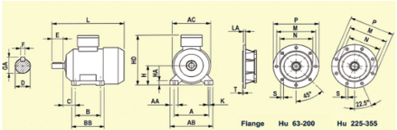
Dimensions of Mounting for Y Series Y 63 - 355
